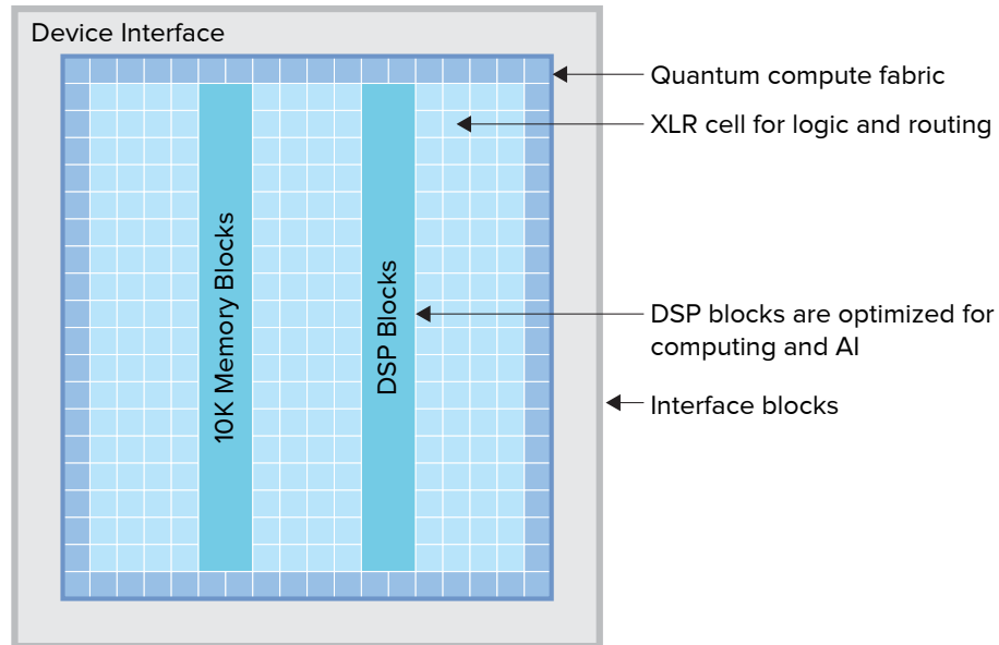
Figure 1: Ti120 FPGA Block Diagram
