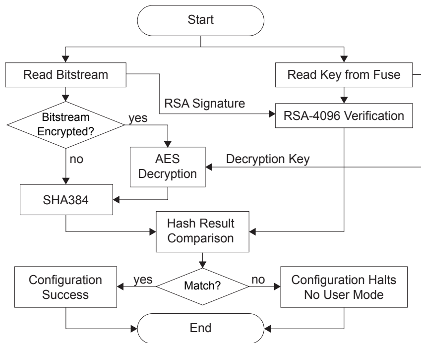
Figure 44: Security Flow
