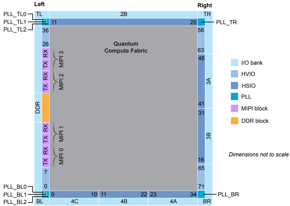
Figure 55: Floorplan Diagram for J484 Packages
