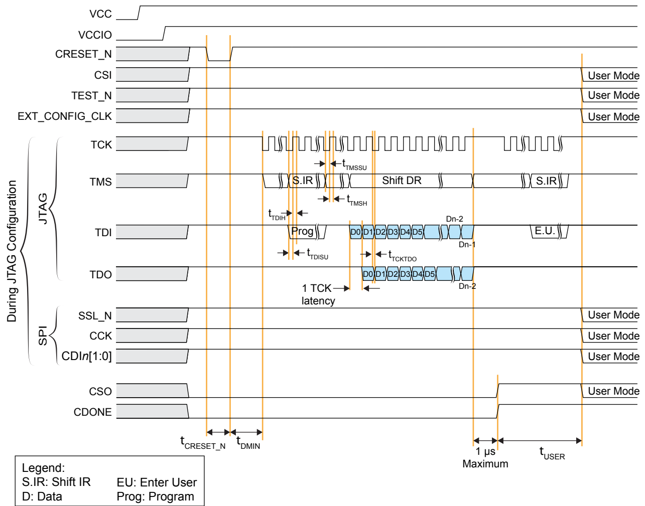
Figure 49: JTAG Timing Waveform
