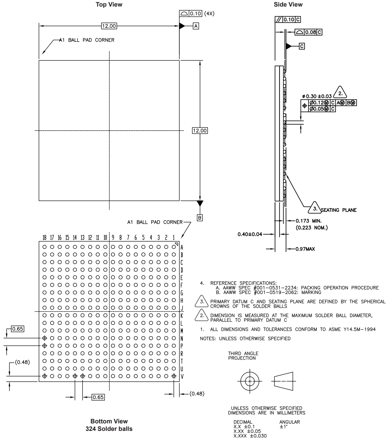
Figure 31: 324-Ball FBGA Package Outline (T20 and T35)
