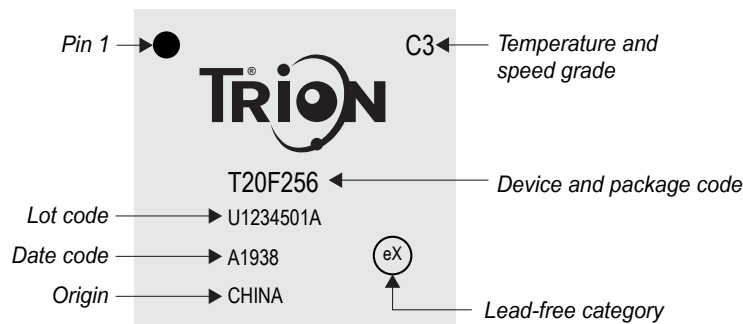
Figure 27: 256-Ball FPGA Package Marking
