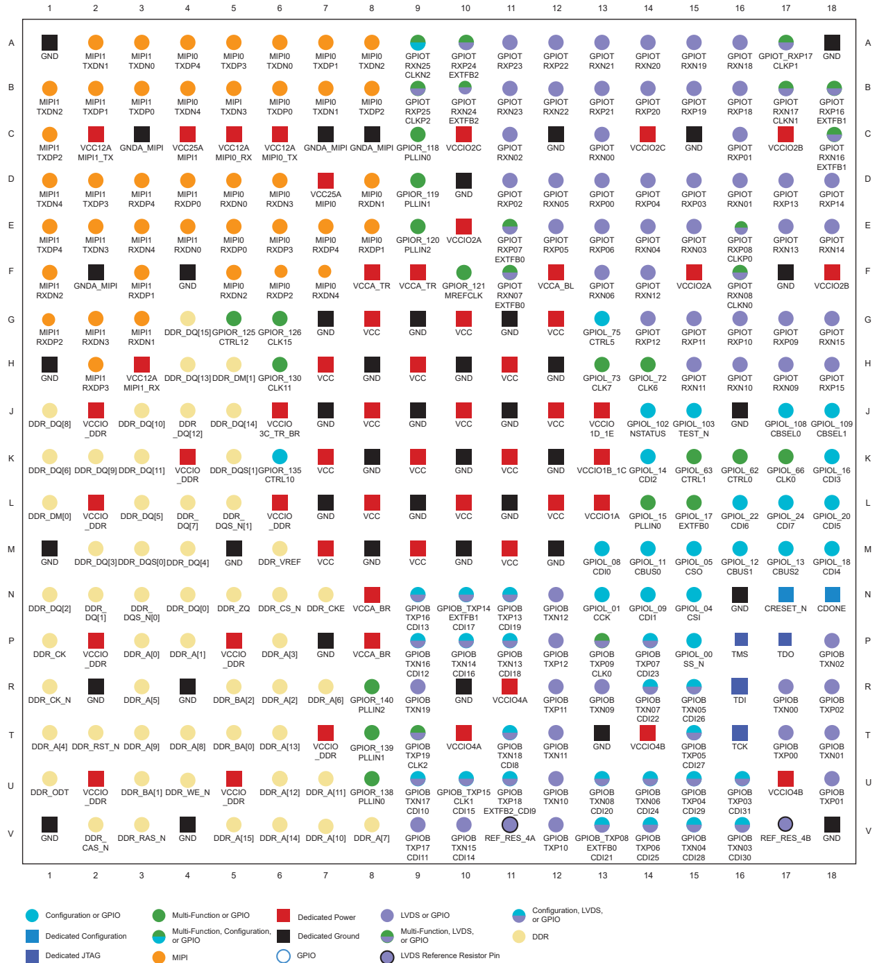
Figure 29: 324-Ball FBGA Pinout Diagram (T20 and T35)
