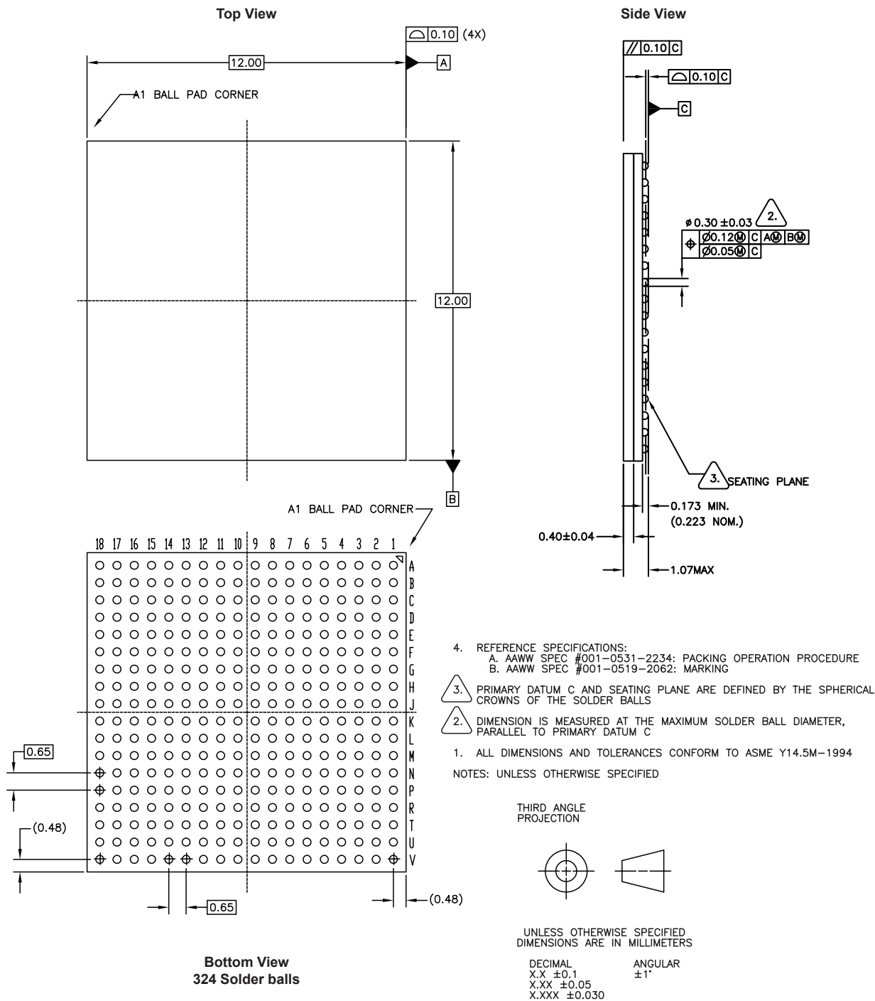
Figure 35: 324-Ball FBGA Package Outline (T55, T85, and T120)
