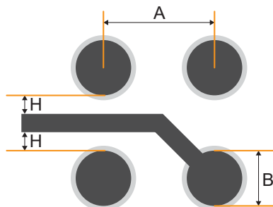
Figure 51: Routing Traces between Pads on the Top Layer
