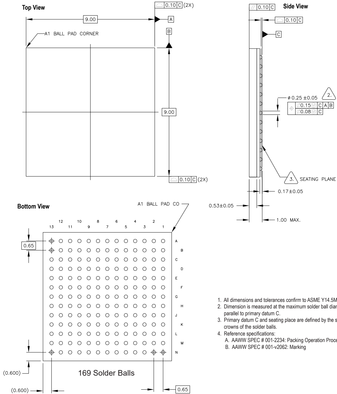
Figure 24: 169-Ball FBGA Package Outline
