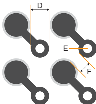
Figure 52: Via Dimensions
