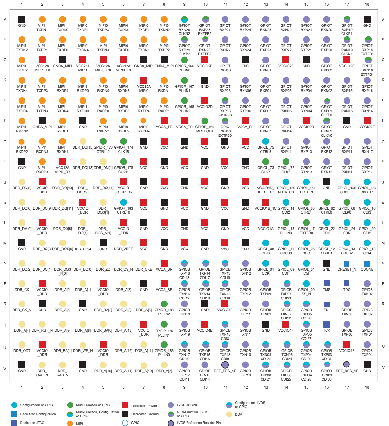
Figure 33: 324-Ball FBGA Pinout Diagram (T55, T85, and T120)
