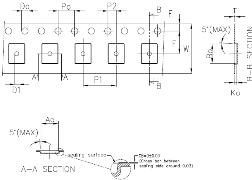
Figure 60: Tape Outline (WLCSP80 Packages)
