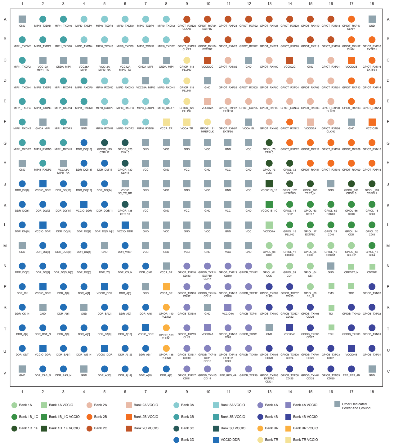
Figure 30: 324-Ball FBGA I/O Bank Diagram (T20 and T35)
