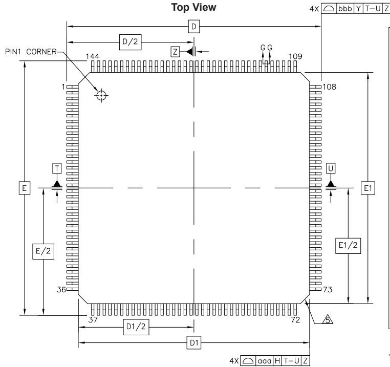
Figure 20: 144-Lead LQFP FPGA Package Outline
