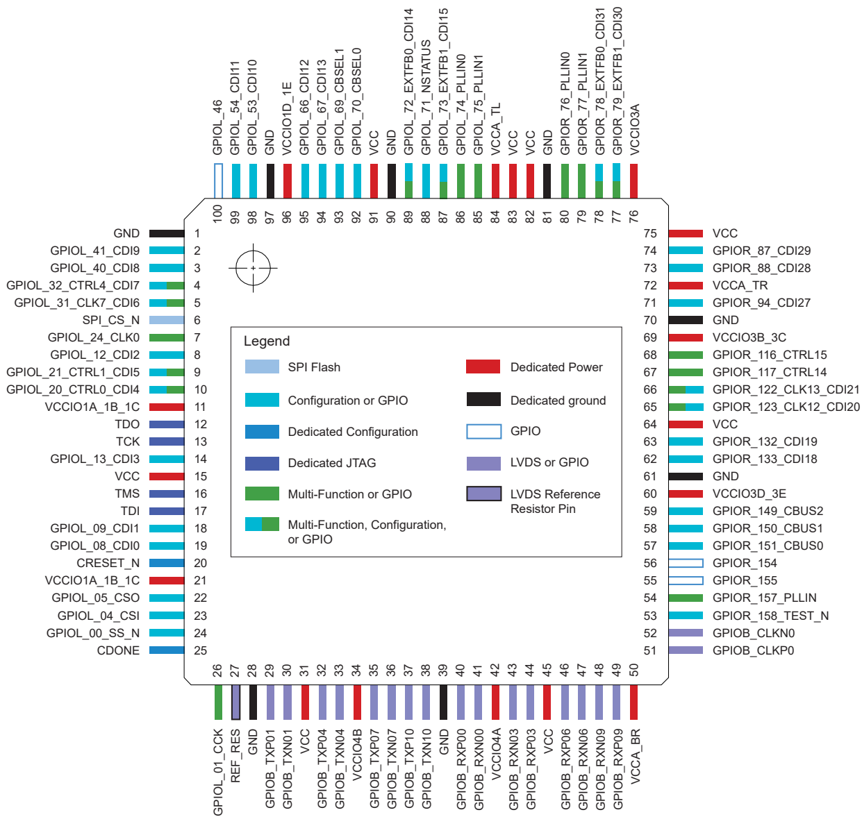
Figure 13: 100-Lead LQFP Pinout Diagram
