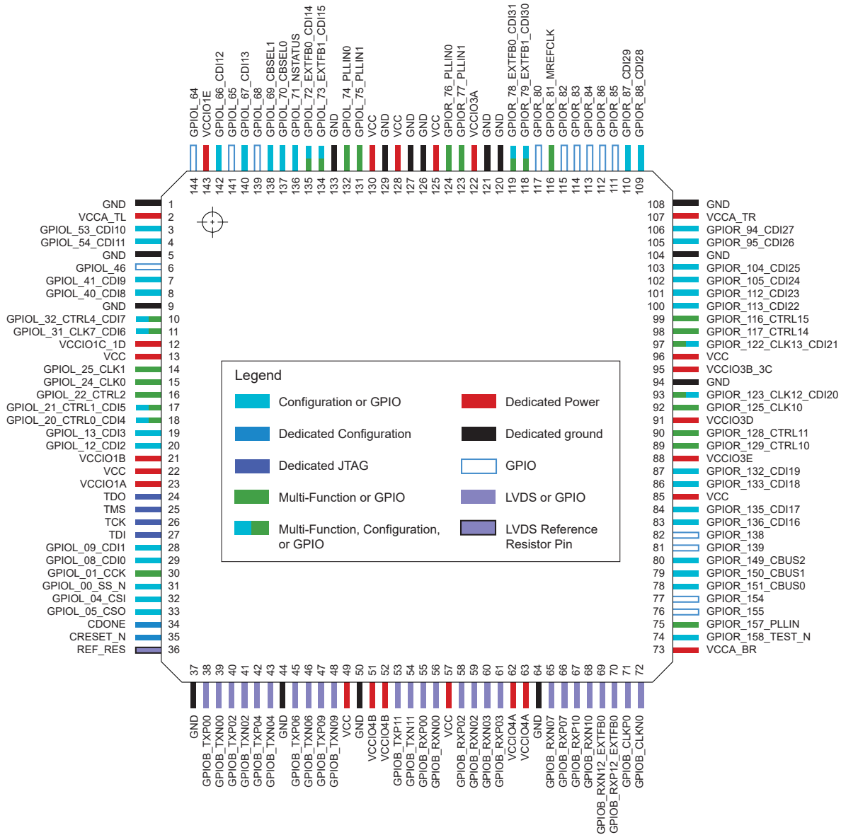
Figure 17: 144-Lead LQFP Pinout Diagram
