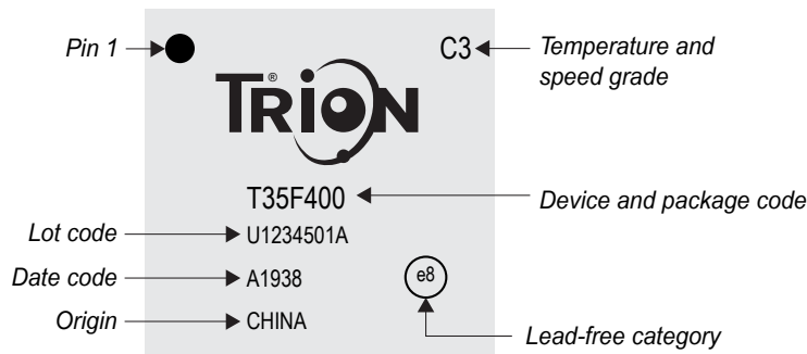
Figure 40: 400-Ball FPGA Package Marking
