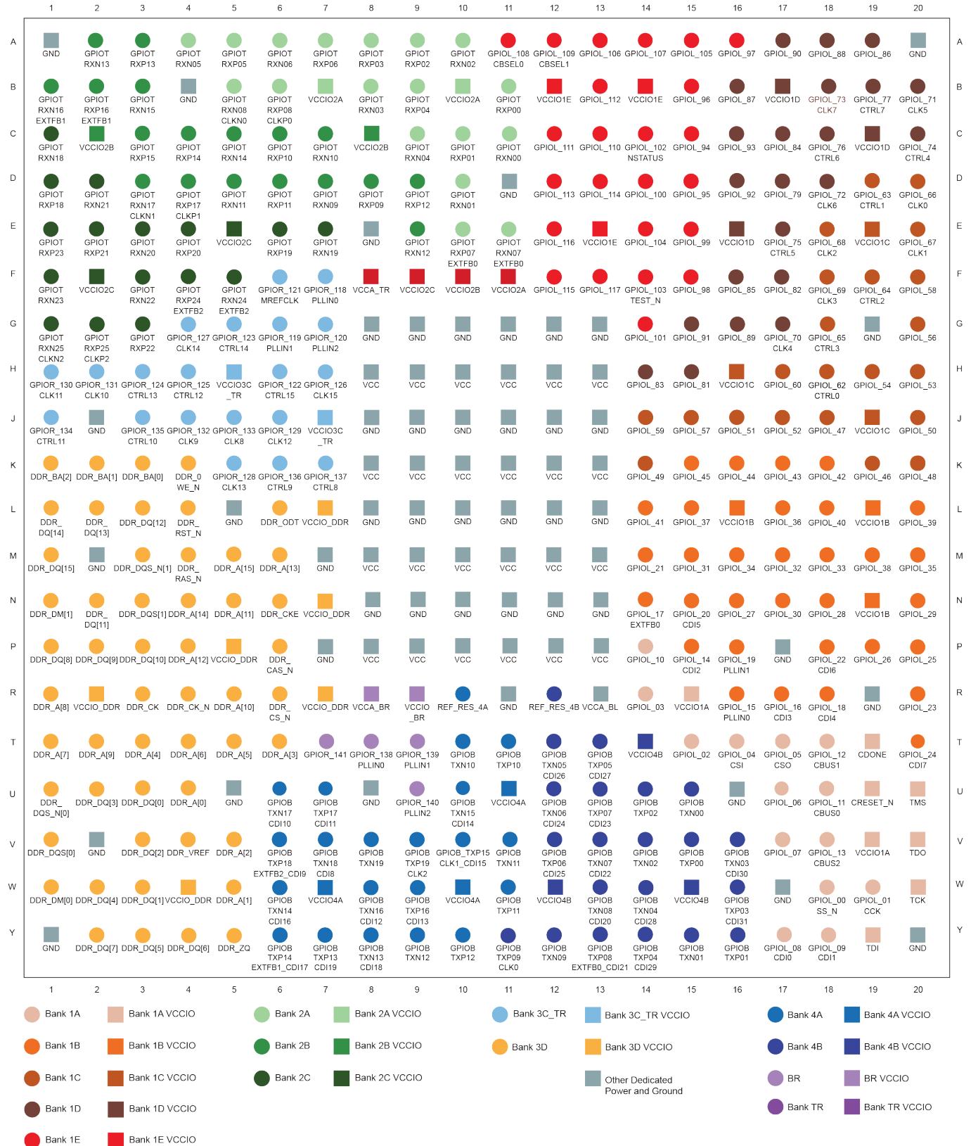
Figure 38: 400-Ball FBGA I/O Bank Diagram
