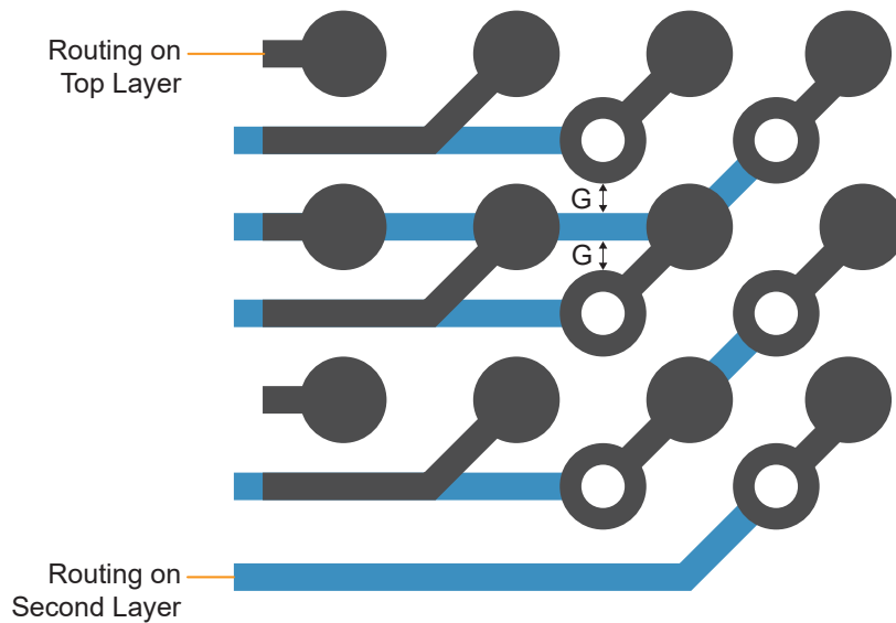
Figure 53: BGA Trace Routing for Top and Second Layers
