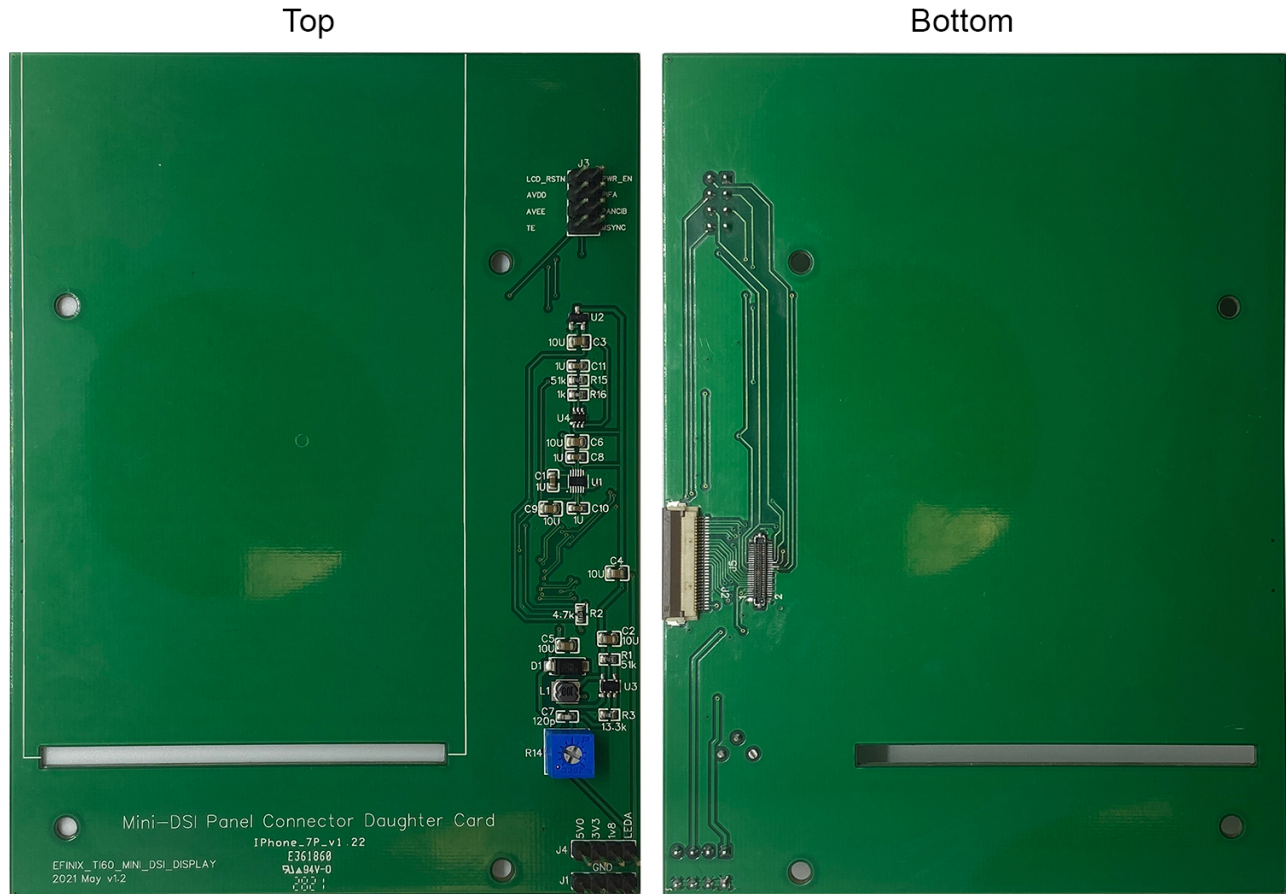
Figure 8: Mini-DSI Panel Connector Daughter Card
