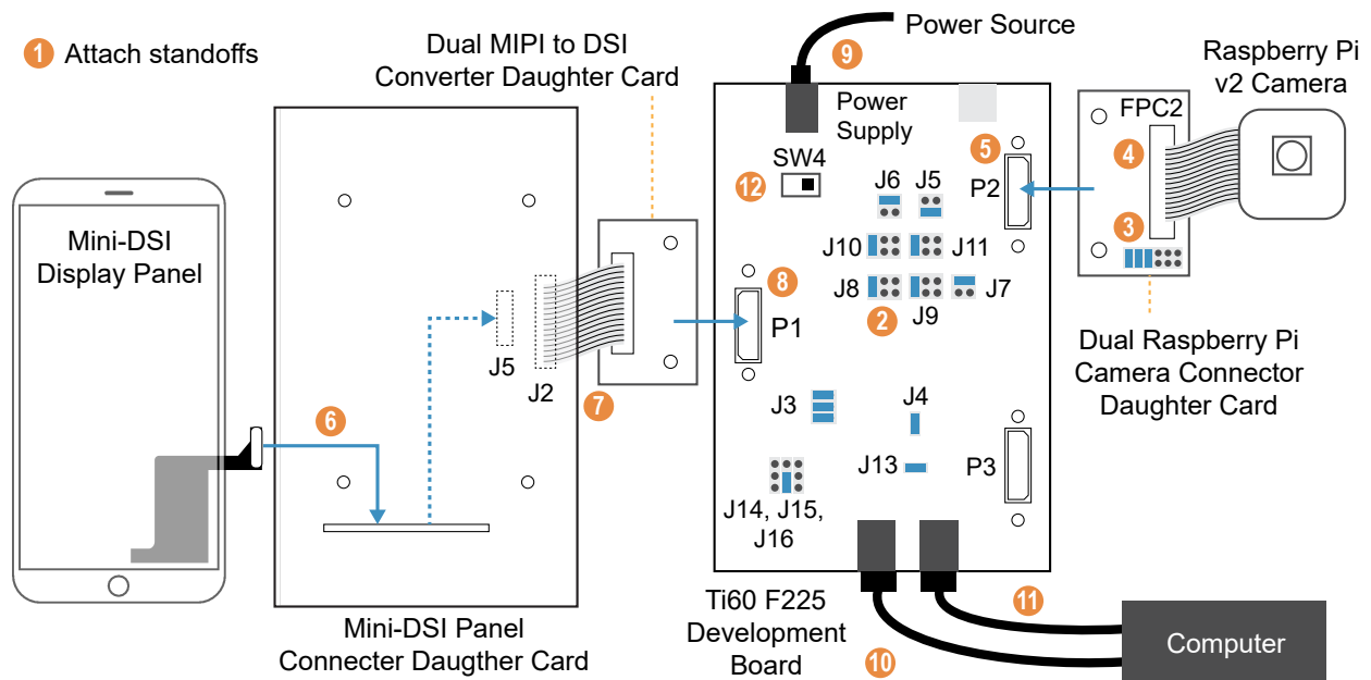
Figure 13: Hardware Setup
