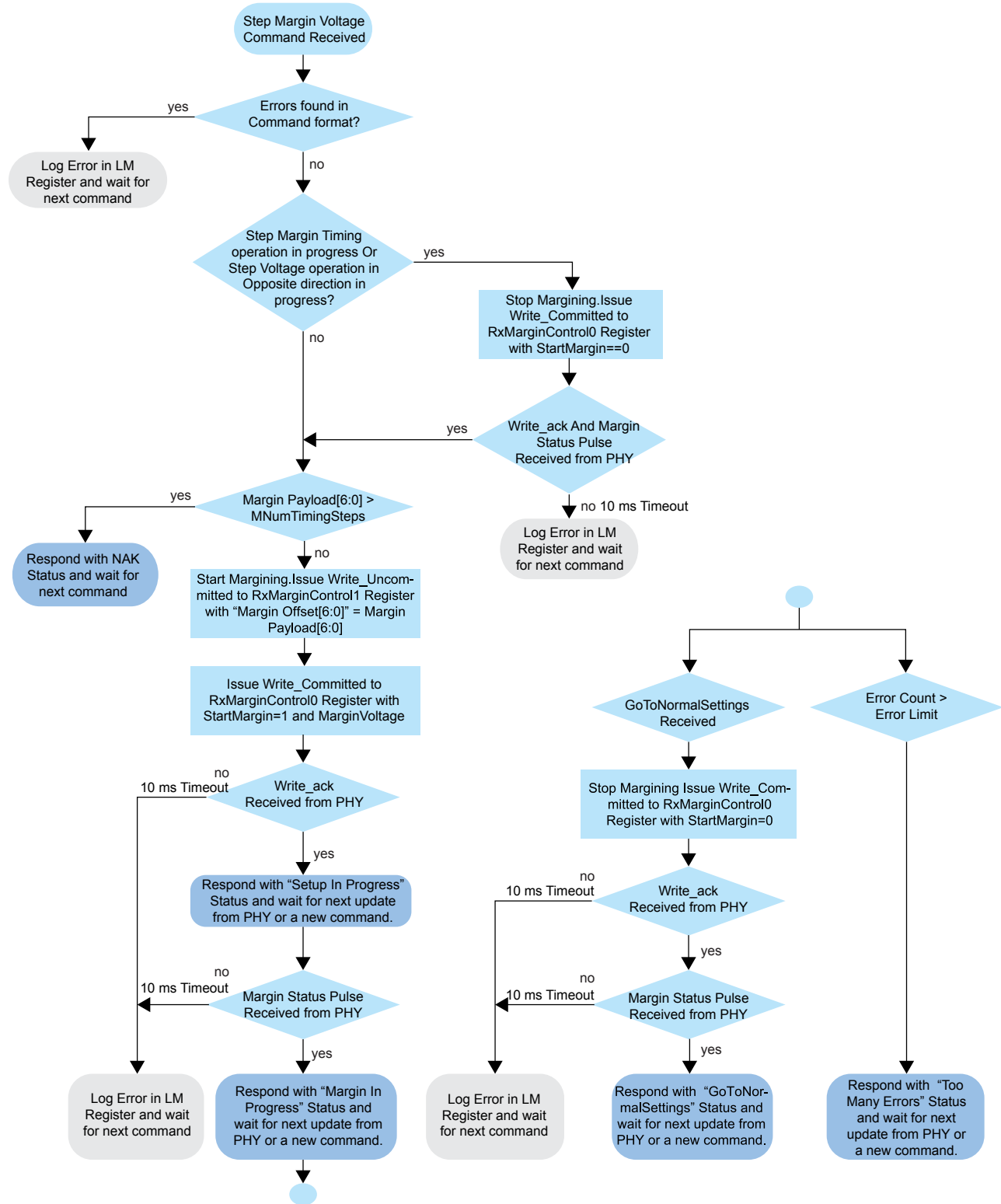
Figure 7: Step Margin for Voltage Command Execution
