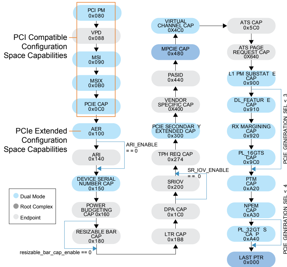
Figure 45: Configuration Capabilities
