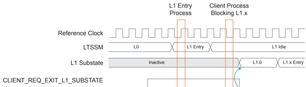
Figure 36: Using CLIENT_REQ_EXIT_L1_SUBSTATE to block L1.x entry
