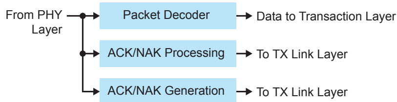
Figure 8: RX Data Link Layer
