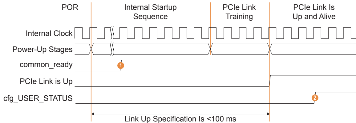
Figure 23: PCIe Controller Link Up Mechanism
