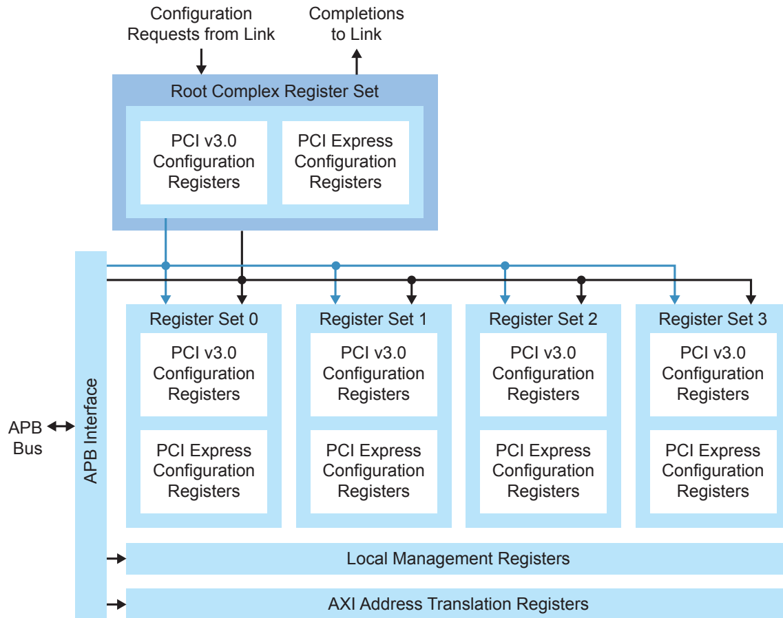
Figure 37: Configuration and Management Registers
