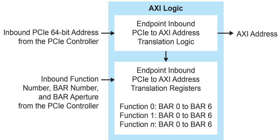
Figure 18: Endpoint Inbound PCIe to AXI Address Translation
