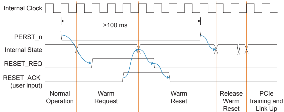
Figure 24: Reset Handshake
