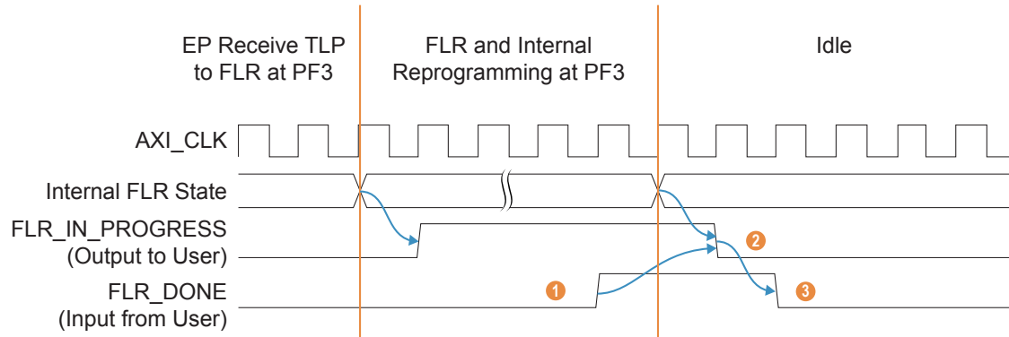
Figure 25: FLR Handshake
