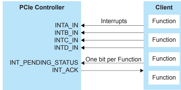
Figure 22: Legacy Endpoint Interrupt Interface
