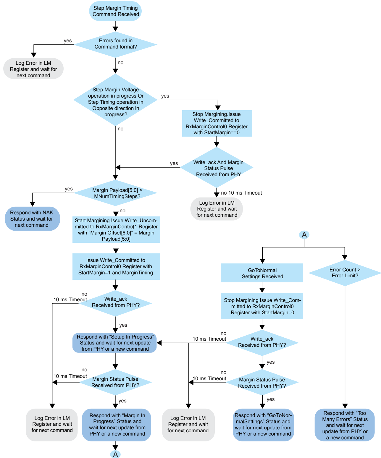
Figure 6: Step Margin for Timing Command Execution
