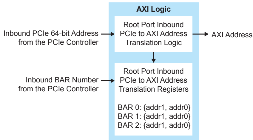
Figure 17: Root Port Inbound PCIe to AXI Address Translation
