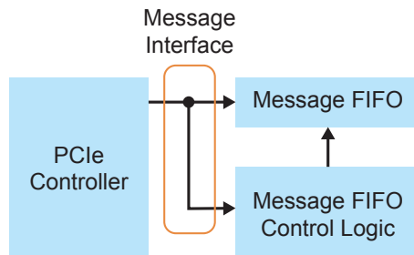
Figure 16: Message Interface FIFO
