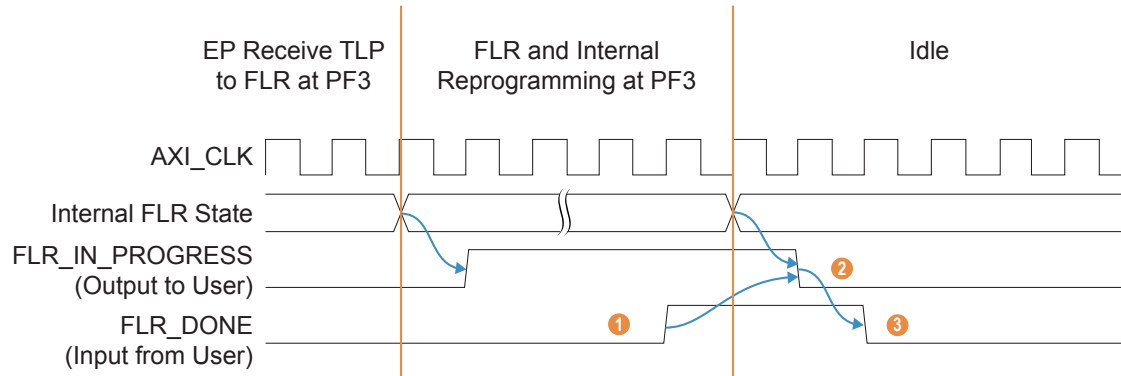
Figure 25: FLR Handshake
