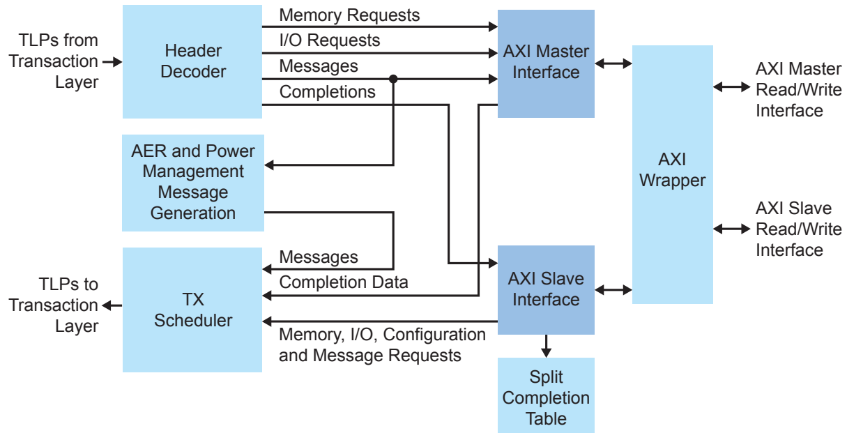
Figure 12: AXI Modules
