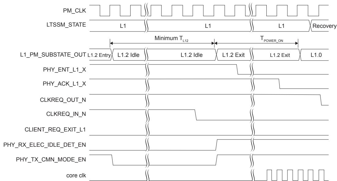
Figure 34: L1.2 Substate Exit Initiated by Link Partner
