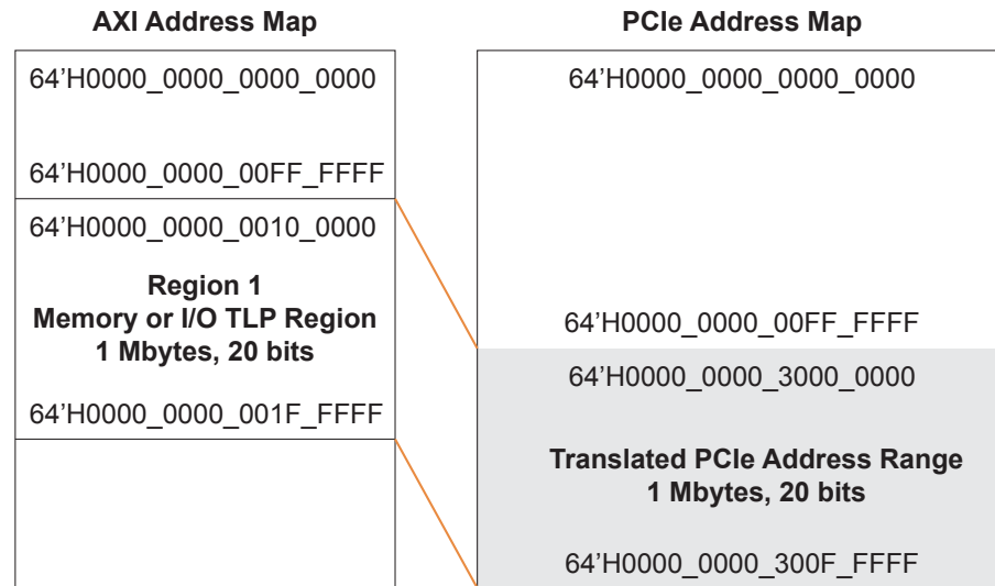
Figure 44: Outbound AXI to PCIe Address Translation Register Programming
