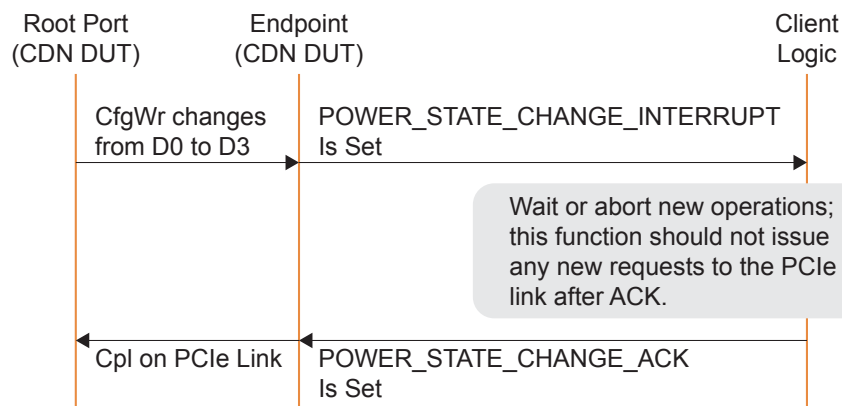
Figure 26: Asserting POWER_STATE_CHANGE_INTERRUPT
