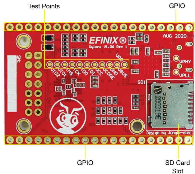
Figure 4: Xyloni Development Board Components (Bottom)
