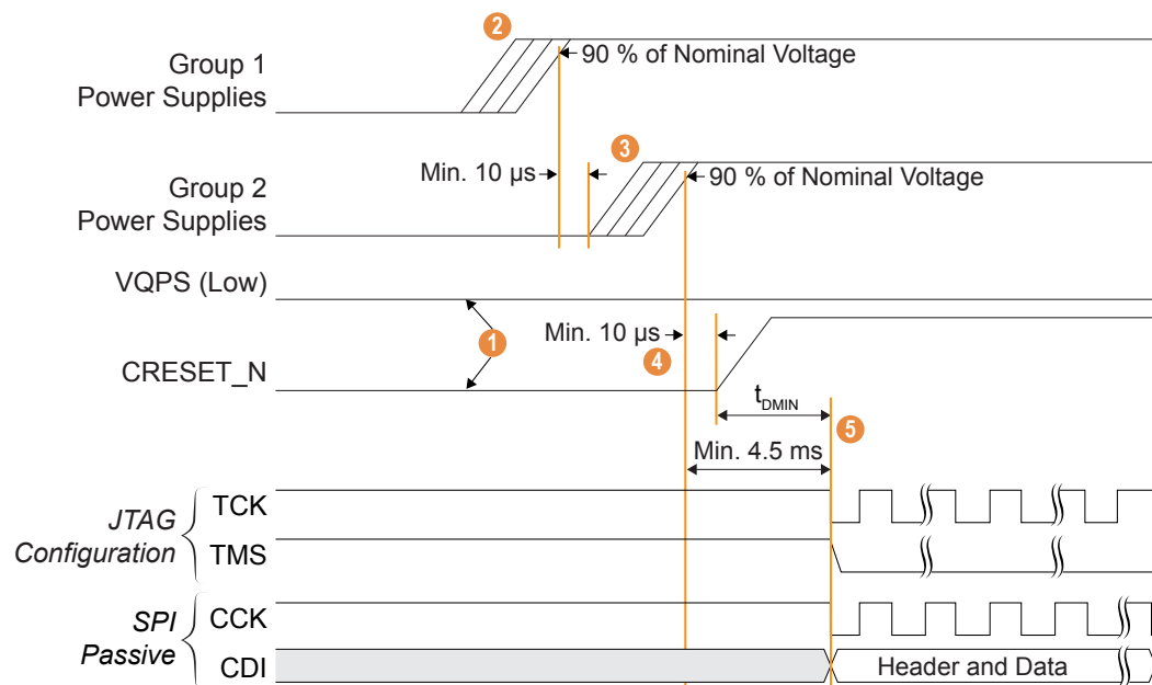
Figure 46: Power-Up Sequence
